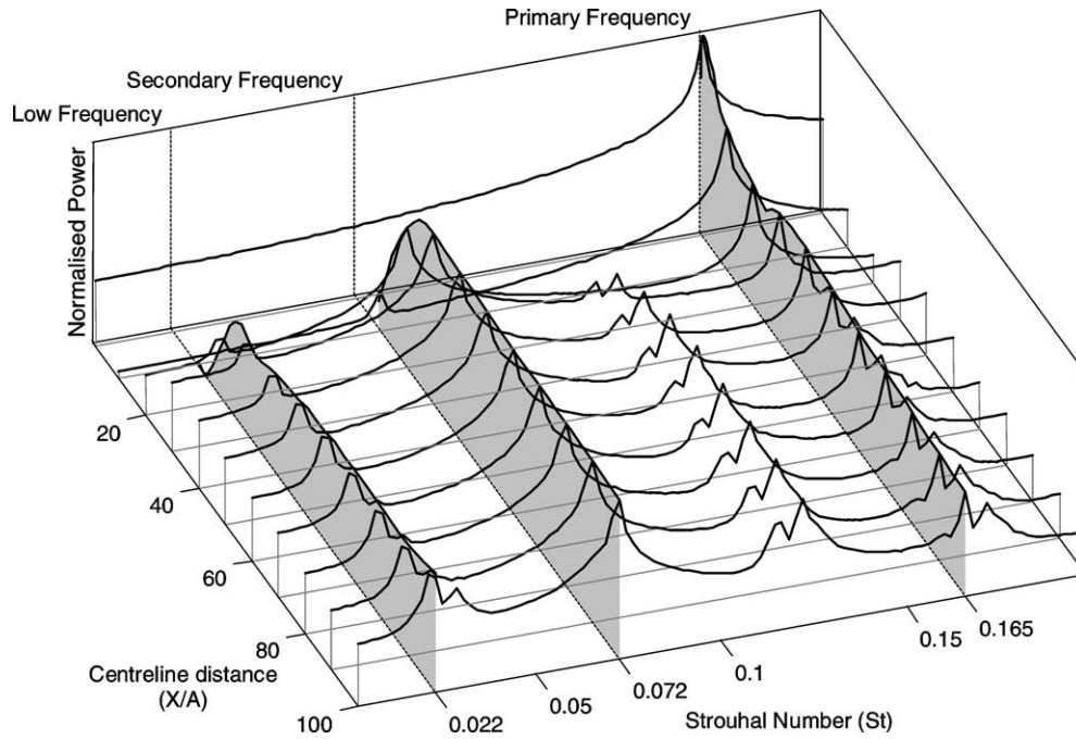
Fig. 14. Normalised power spectra of the transverse velocity component on centreline for AR = 0.25 at Re = 150 .
