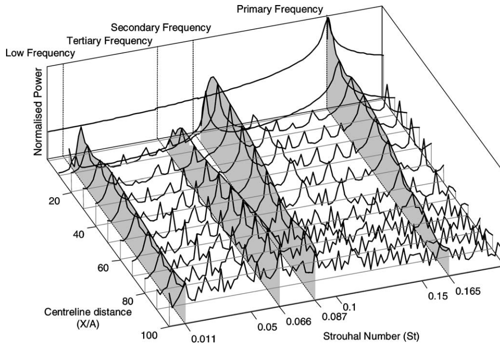
Fig. 16. Normalised power spectra of the transverse velocity component on centreline for AR = 0.25 at Re = 175 .
